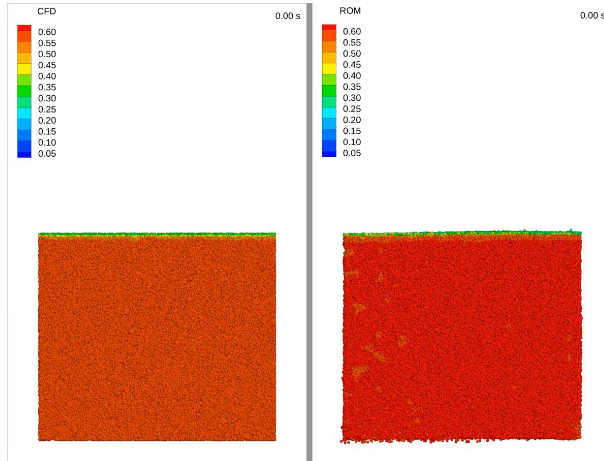
CFD – Reference
