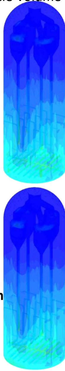
Particle Volume-fraction
