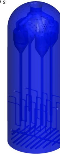
CFD – Reference
