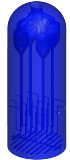
GNN-ROM – Prediction
