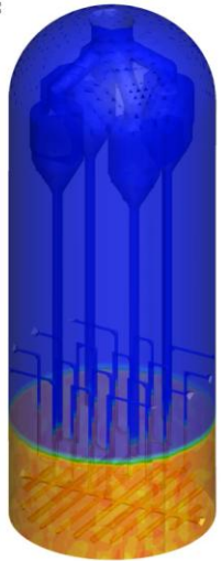
CFD – Reference
