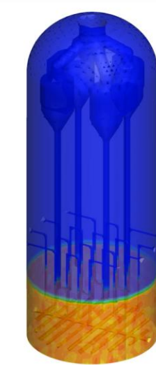
GNN-ROM – Prediction
